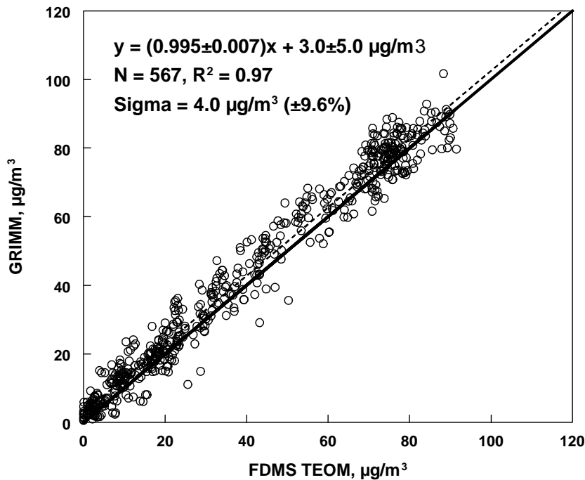
Figure 1. Comparison of PM 2.5 hourly average mass measurements by an FDMS-TEOM and a GRIMM monitor for the 19 January through 16 February 2007 study at Lindon, Utah. The linear regression fit to the results are given in the Figure
