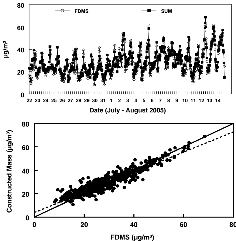
Figure 2. Semi-continuous constructed mass (y axis in both plots) vs. FDMS measured mass. Constructed mass is the sum of all the major components of the aerosol including; NVOM, SVOM, EC, NH 4 NO 3 and ammonium sulfate.
