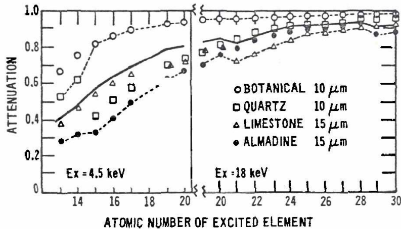
Figure C. Attenuation factors for K α X-rays of various elements calculated for four different coarse particle compositions (from Dzubay and Nelson, 1975).
