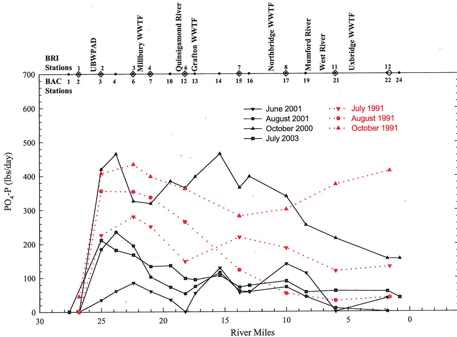
Figure 31. PO 4 -P Loading Profiles for the BRI 1991 and BAC 2000-3 Surveys
